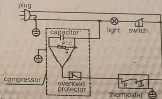
DIAGRAM OF CIRCUIT PRINCIPLE
