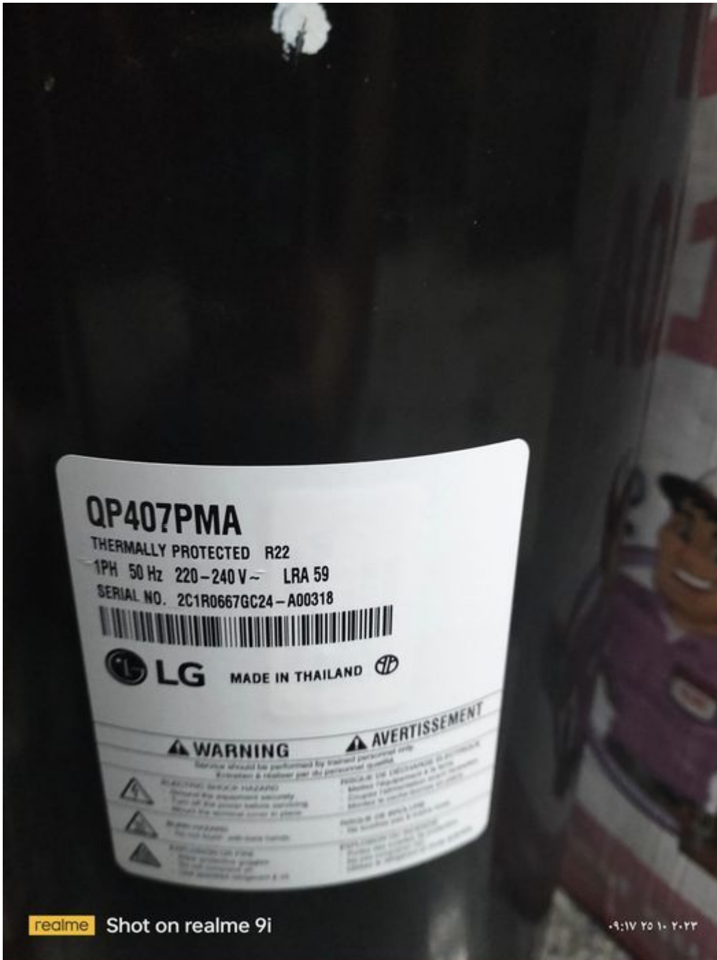
Compressor, LG, QP407PMA, 2.5 hp, r22, 24045 btu, 7048 w
